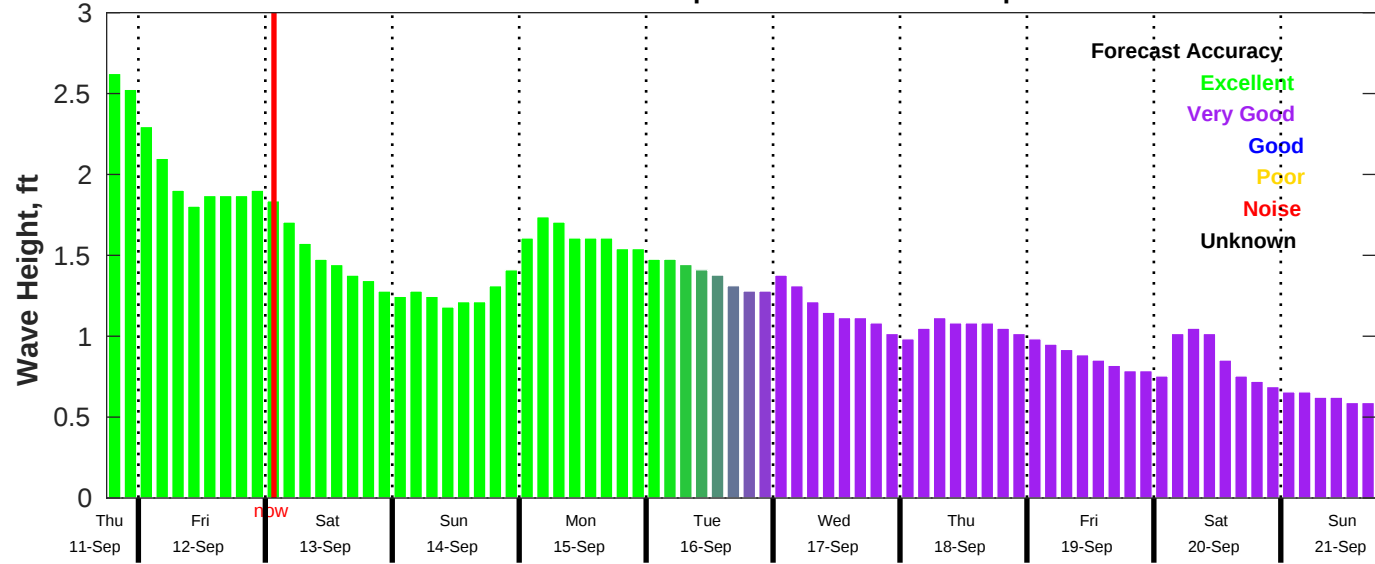
CMEMS Wave Forecast for NDBC 42035 from 11-Sep-2025 18:00:00 to 21-Sep-2025 18:00:00
