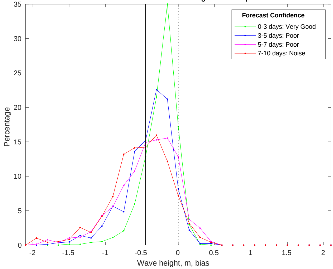
NDBC 42036 vs CMEMS Waves Bias Histogram: 13-Sep-2025
