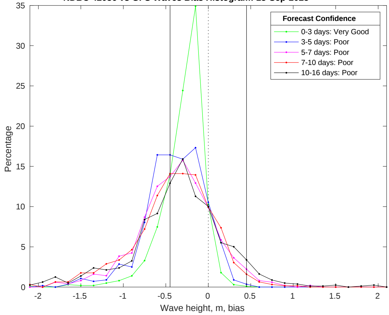
NDBC 42036 vs GFS Waves Bias Histogram: 13-Sep-2025
