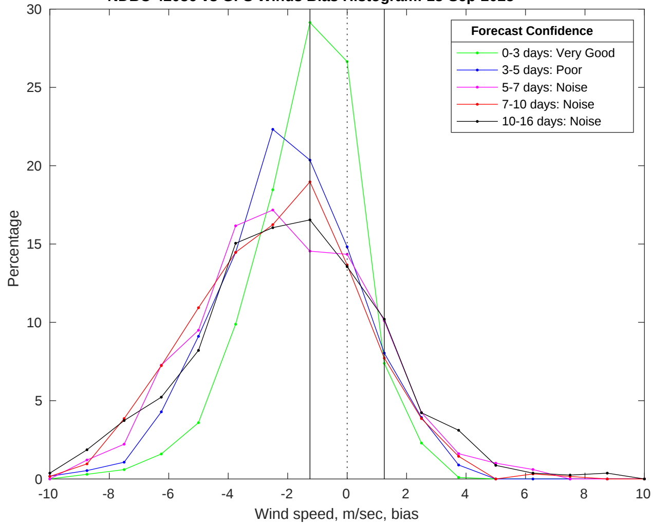
NDBC 42036 vs GFS Winds Bias Histogram: 13-Sep-2025
