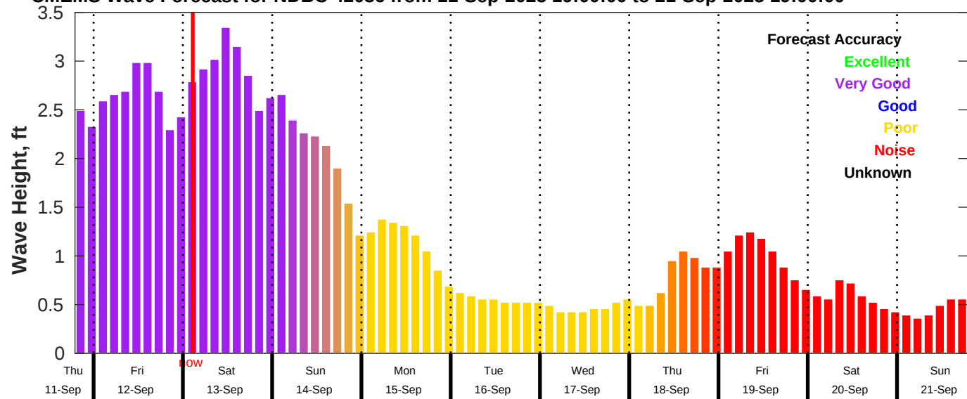
CMEMS Wave Forecast for NDBC 42036 from 11-Sep-2025 19:00:00 to 21-Sep-2025 19:00:00
