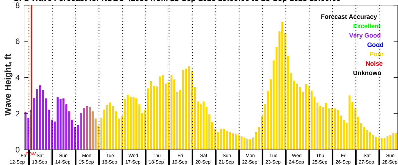
GFS Wave Forecast for NDBC 42036 from 12-Sep-2025 19:00:00 to 28-Sep-2025 19:00:00
