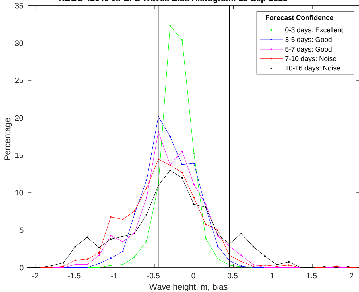
NDBC 42040 vs GFS Waves Bias Histogram: 13-Sep-2025
