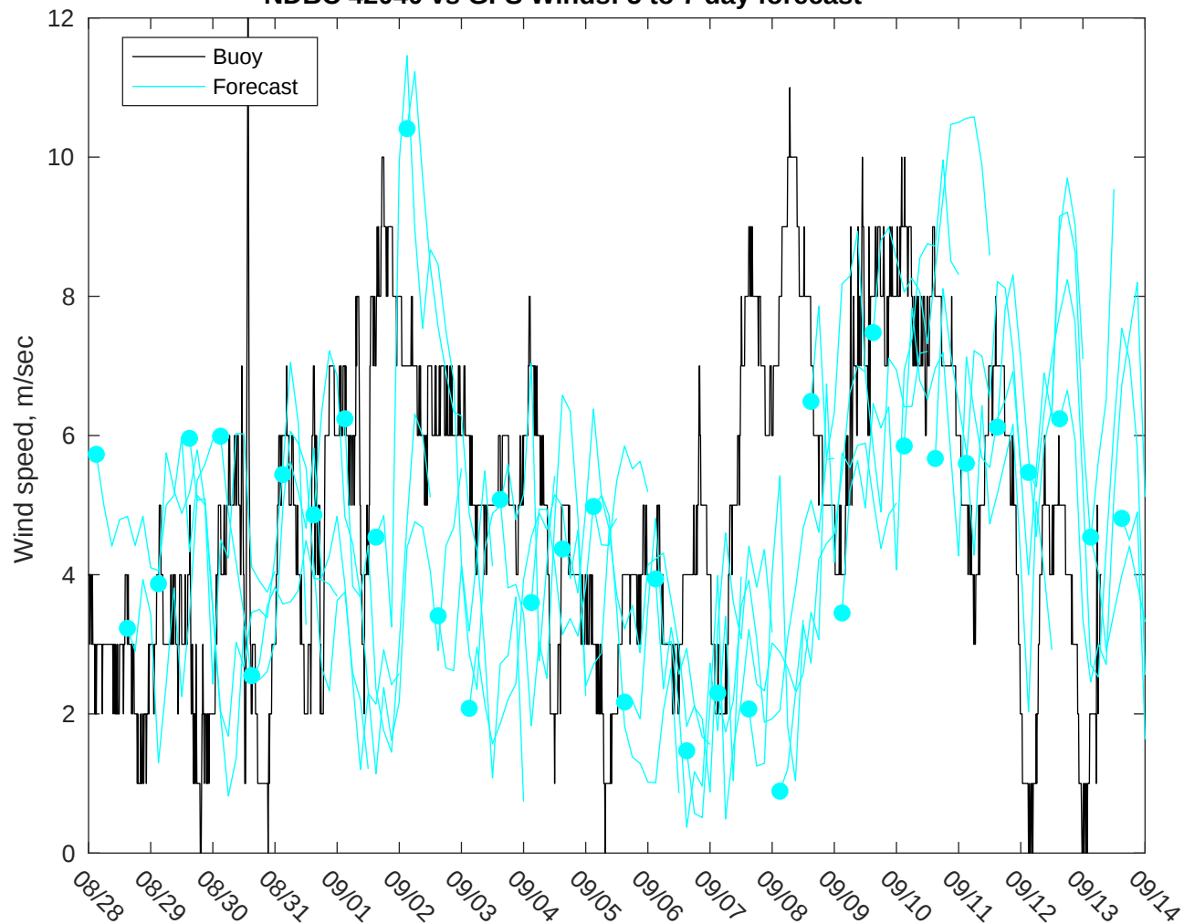
NDBC 42040 vs GFS Winds: 5 to 7 day forecast
