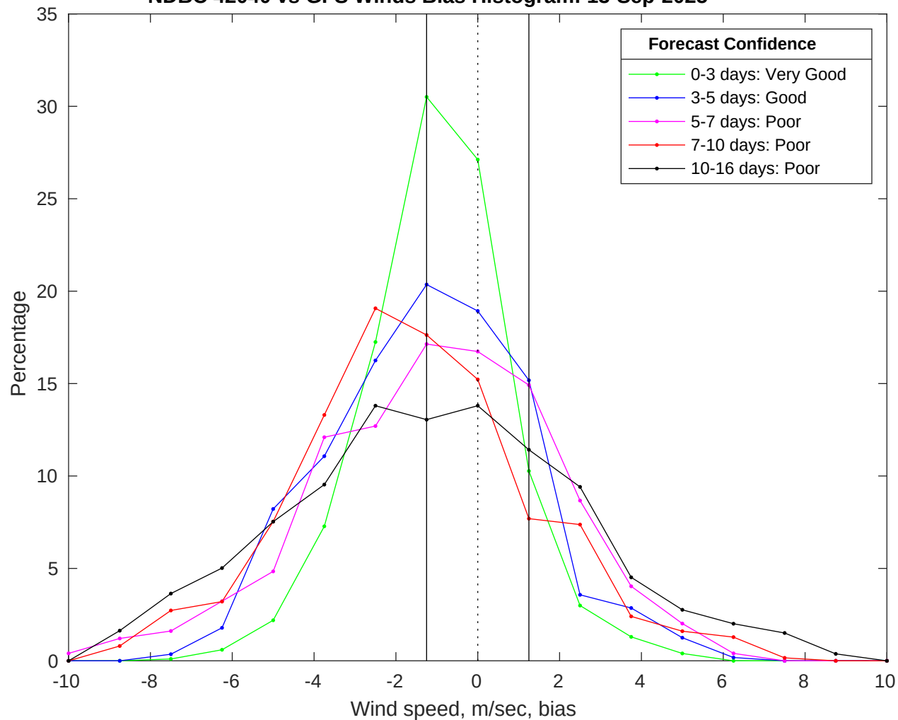
NDBC 42040 vs GFS Winds Bias Histogram: 13-Sep-2025
