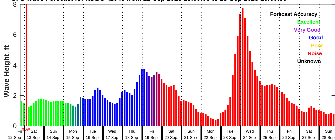
GFS Wave Forecast for NDBC 42040 from 12-Sep-2025 19:00:00 to 28-Sep-2025 19:00:00
