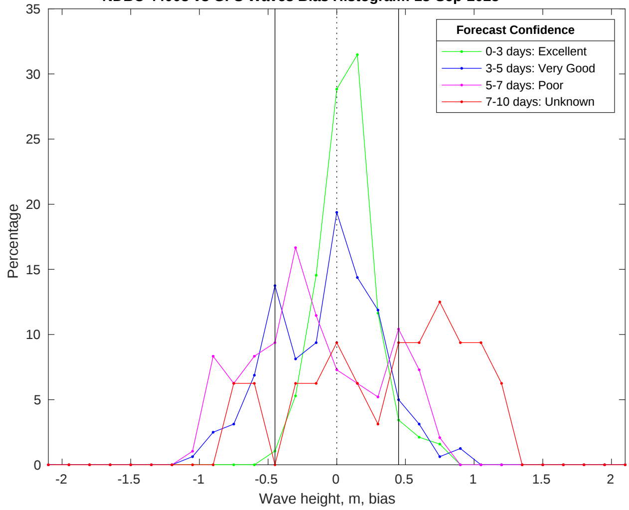
NDBC 44008 vs GFS Waves Bias Histogram: 13-Sep-2025
