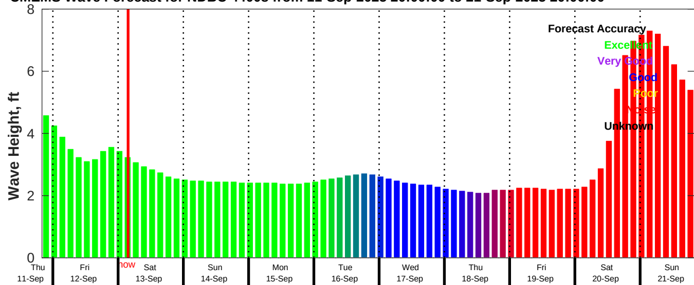
CMEMS Wave Forecast for NDBC 44008 from 11-Sep-2025 20:00:00 to 21-Sep-2025 20:00:00
