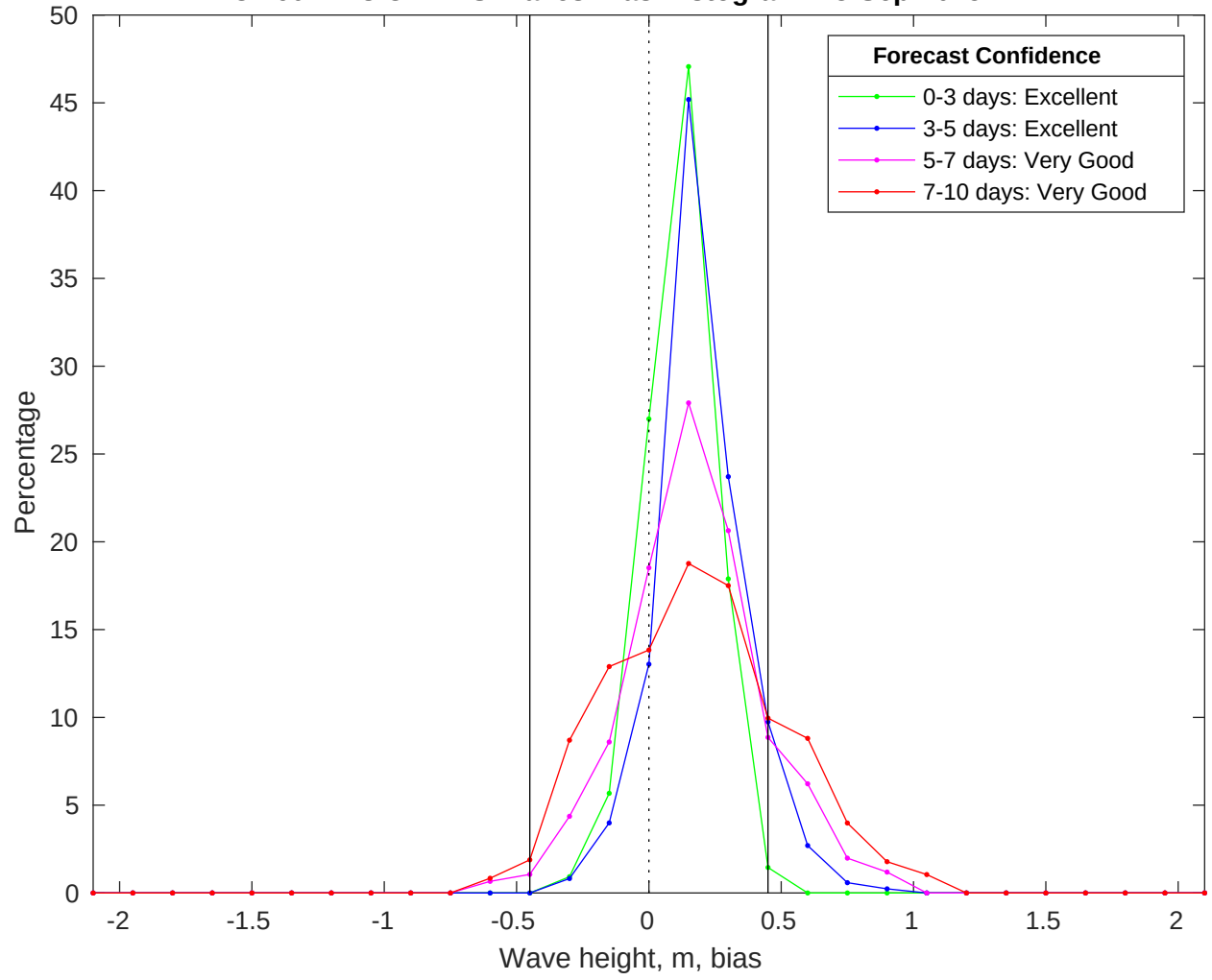
NDBC 46011 vs CMEMS Waves Bias Histogram: 13-Sep-2025
