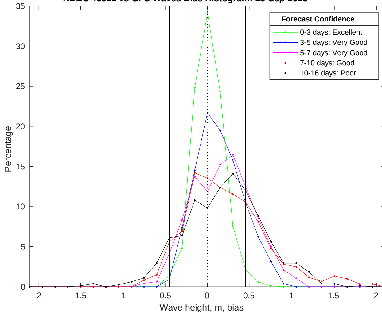
NDBC 46011 vs GFS Waves Bias Histogram: 13-Sep-2025
