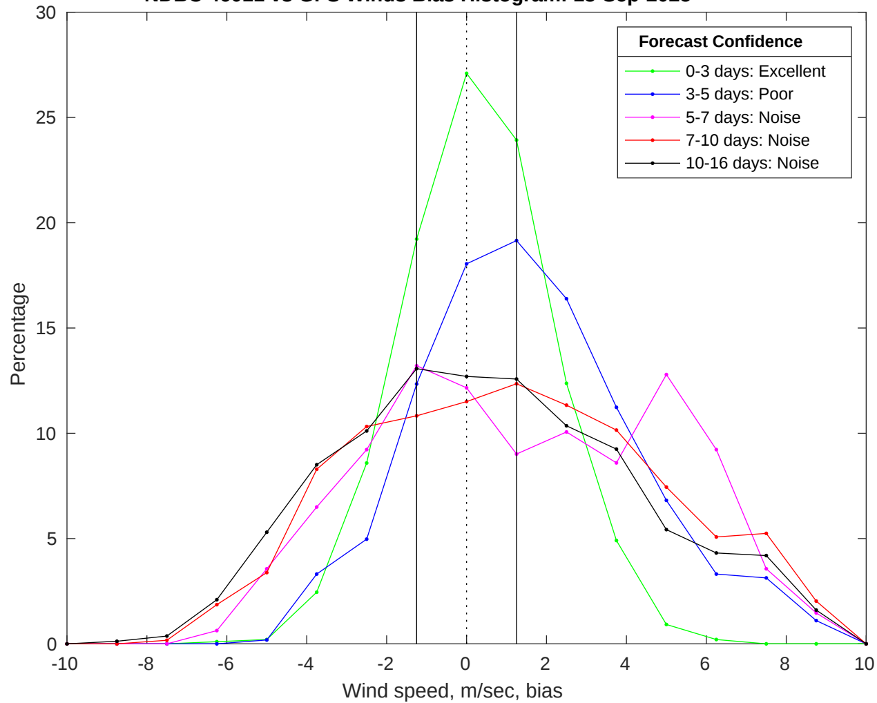
NDBC 46011 vs GFS Winds Bias Histogram: 13-Sep-2025
