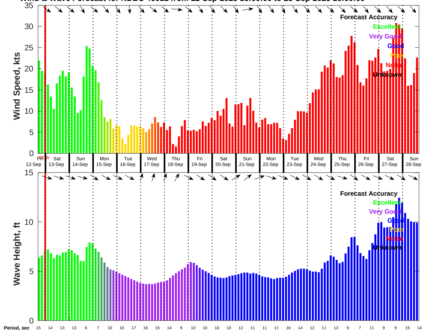
Wind & Wave Forecast for NDBC 46011 from 12-Sep-2025 16:00:00 to 28-Sep-2025 16:00:00
