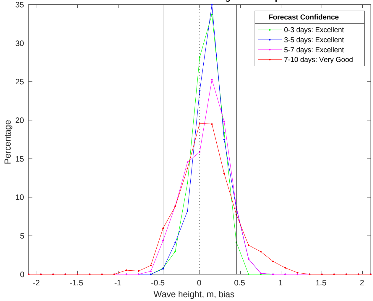
NDBC 46028 vs CMEMS Waves Bias Histogram: 13-Sep-2025
