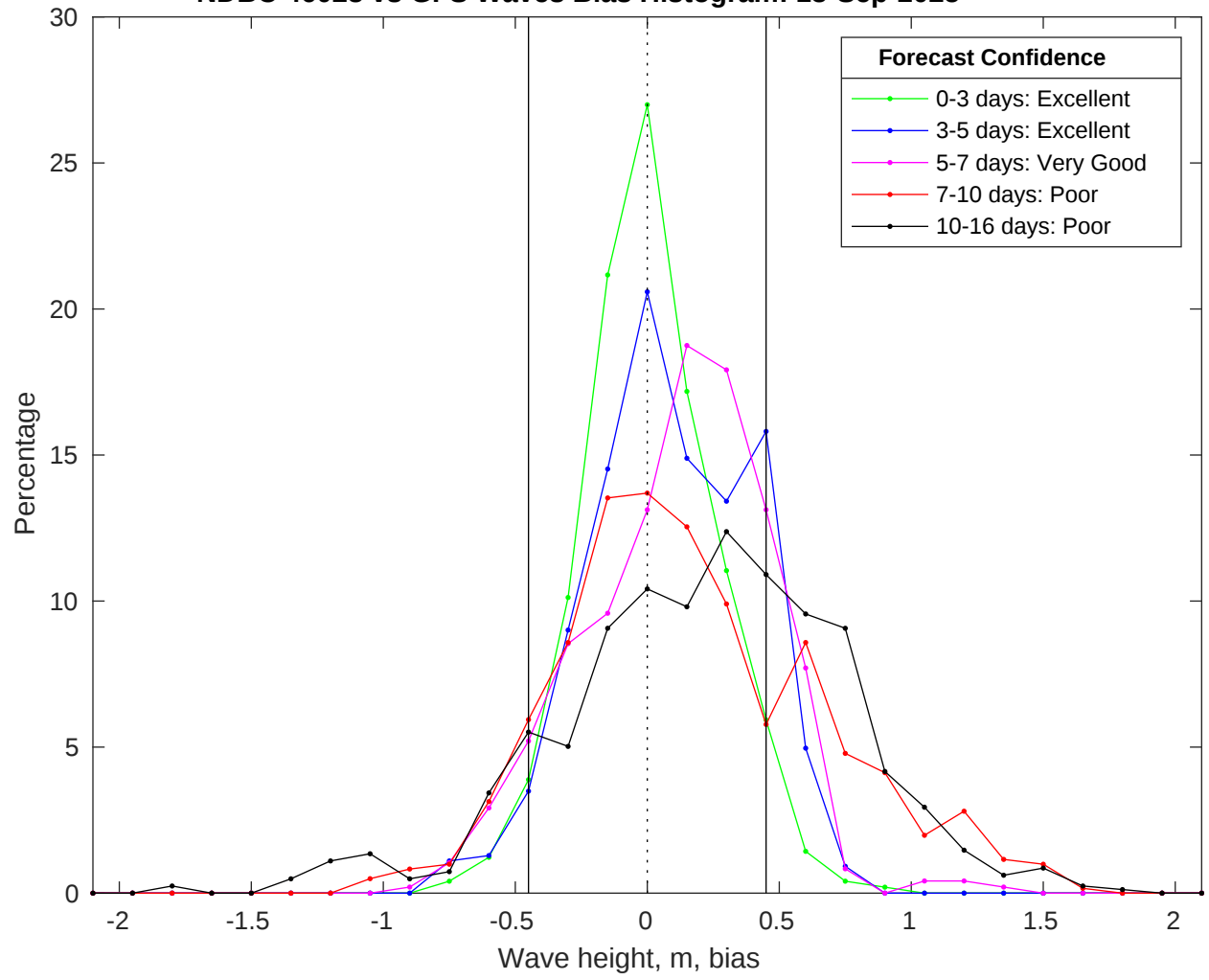
NDBC 46028 vs GFS Waves Bias Histogram: 13-Sep-2025
