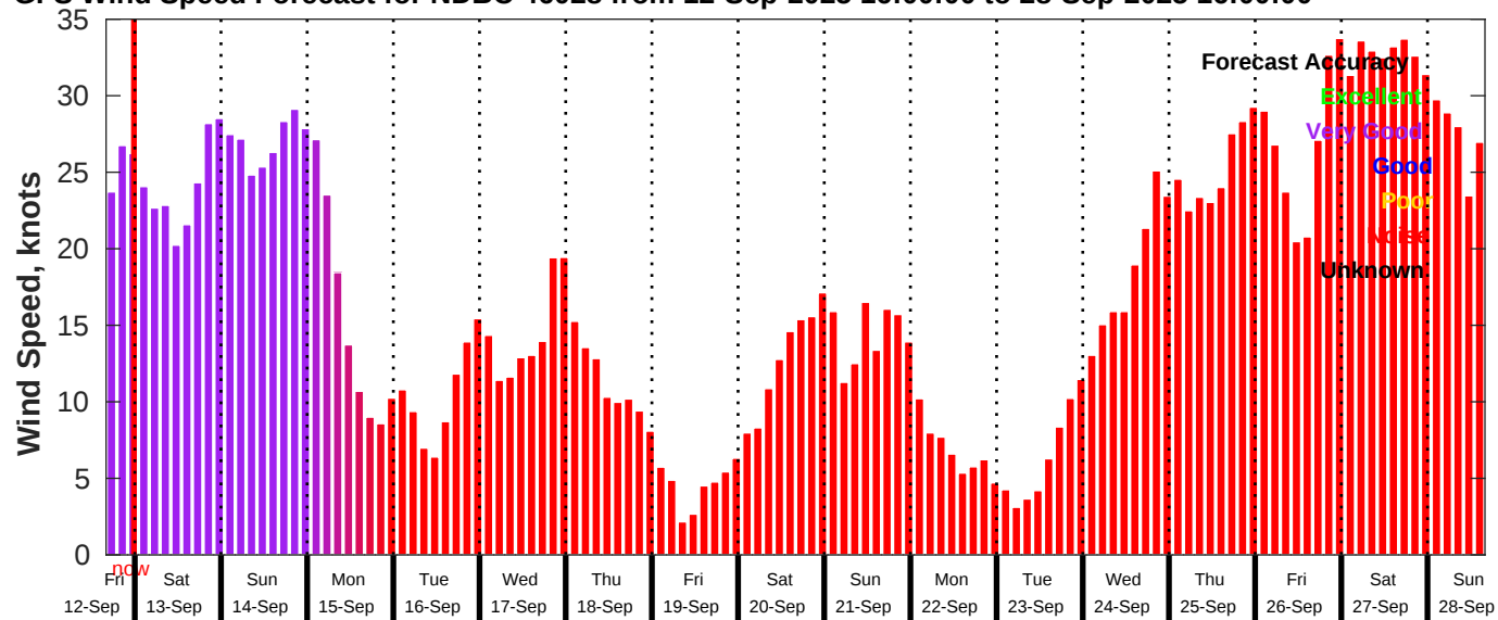
GFS Wind Speed Forecast for NDBC 46028 from 12-Sep-2025 16:00:00 to 28-Sep-2025 16:00:00
