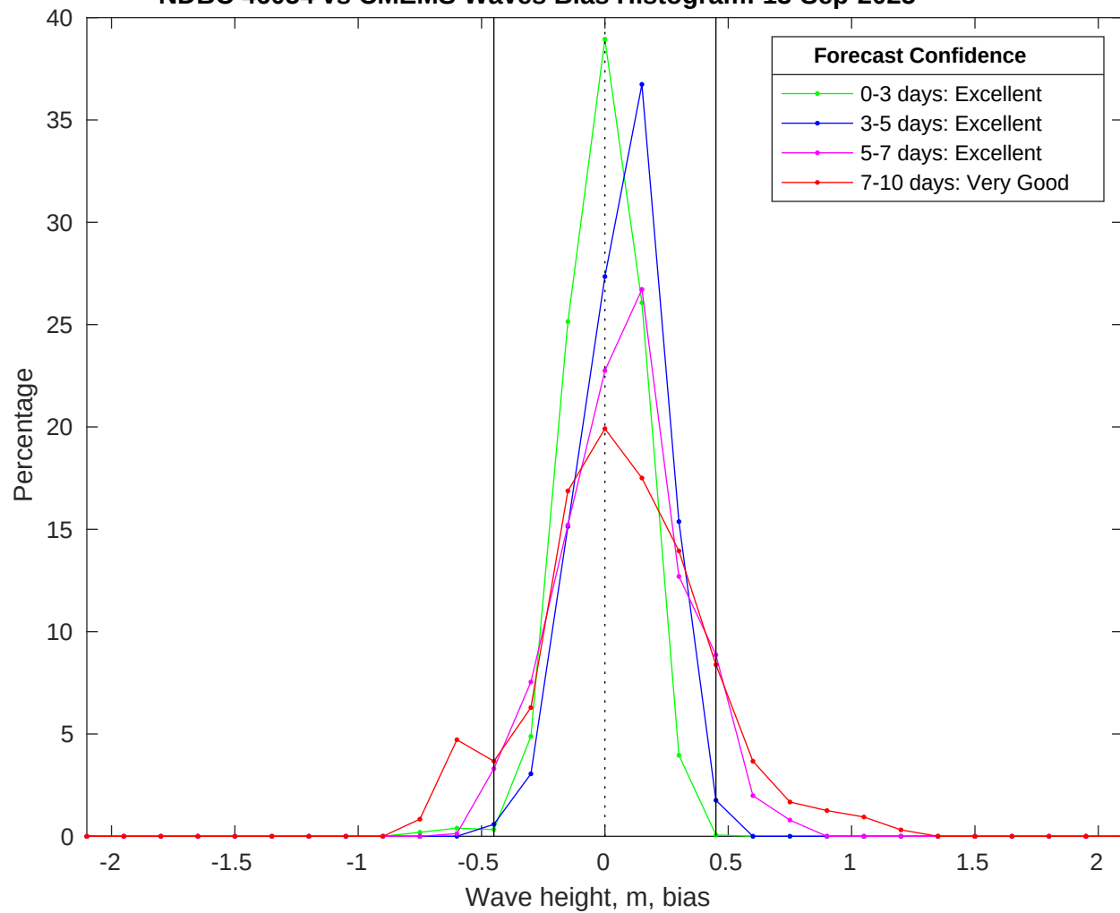
NDBC 46054 vs CMEMS Waves Bias Histogram: 13-Sep-2025
