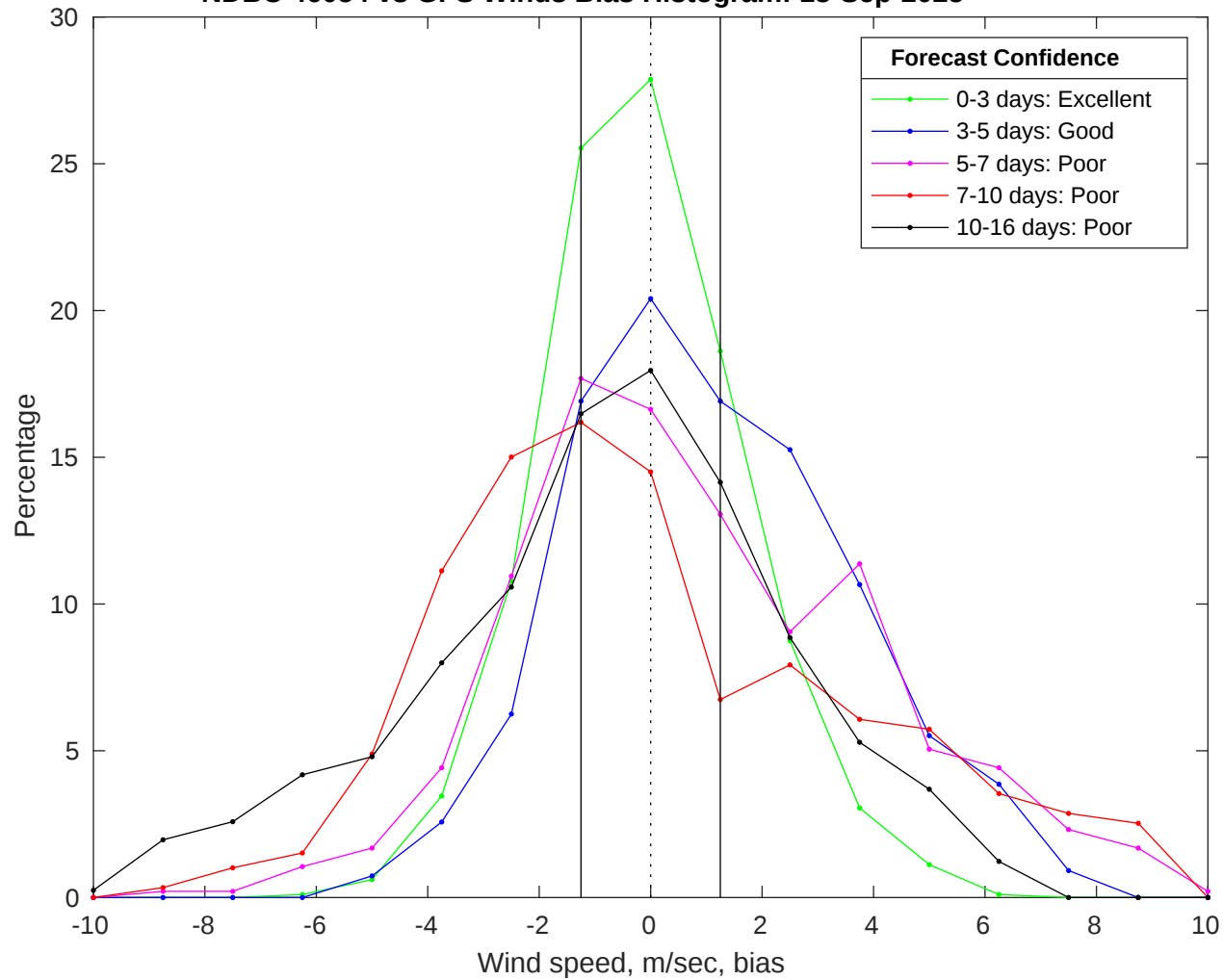
NDBC 46054 vs GFS Winds Bias Histogram: 13-Sep-2025
