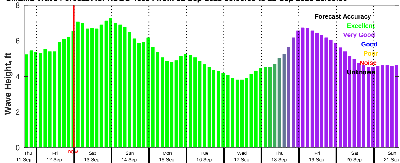
CMEMS Wave Forecast for NDBC 46054 from 11-Sep-2025 16:00:00 to 21-Sep-2025 16:00:00
