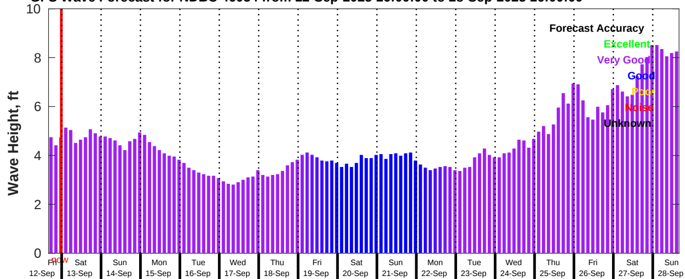
GFS Wave Forecast for NDBC 46054 from 12-Sep-2025 16:00:00 to 28-Sep-2025 16:00:00
