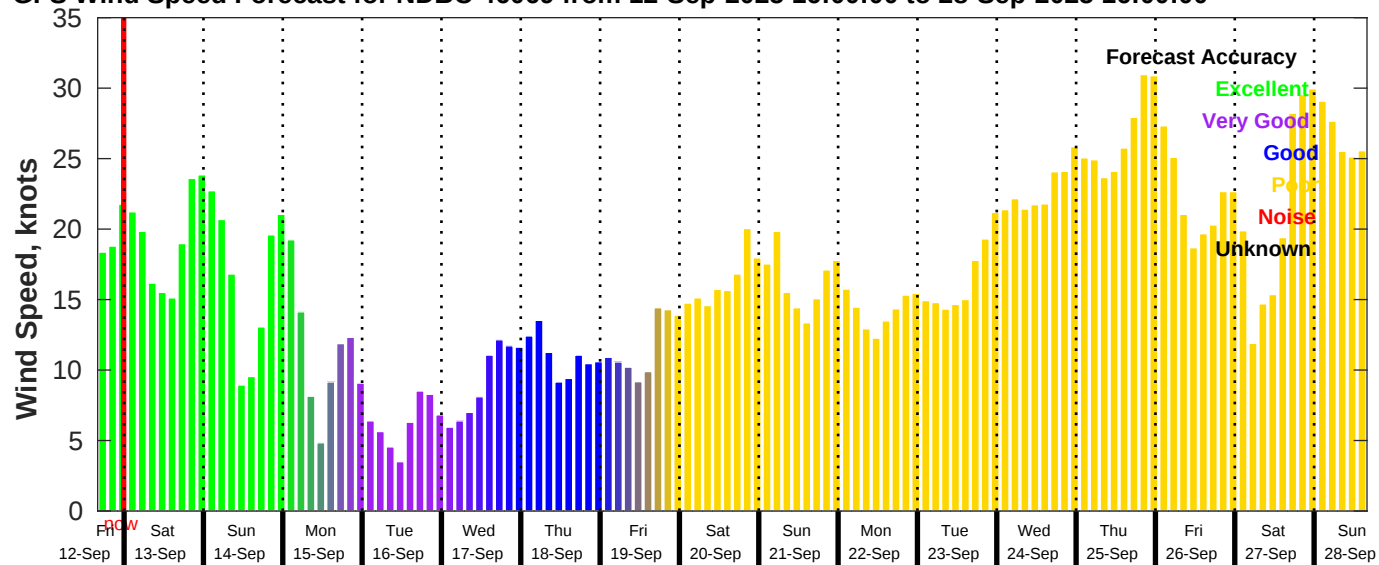
GFS Wind Speed Forecast for NDBC 46069 from 12-Sep-2025 16:00:00 to 28-Sep-2025 16:00:00
