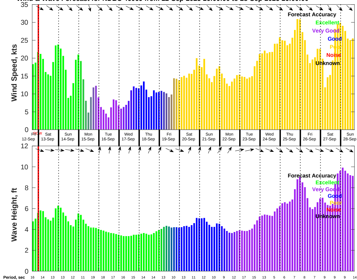
Wind & Wave Forecast for NDBC 46069 from 12-Sep-2025 16:00:00 to 28-Sep-2025 16:00:00
