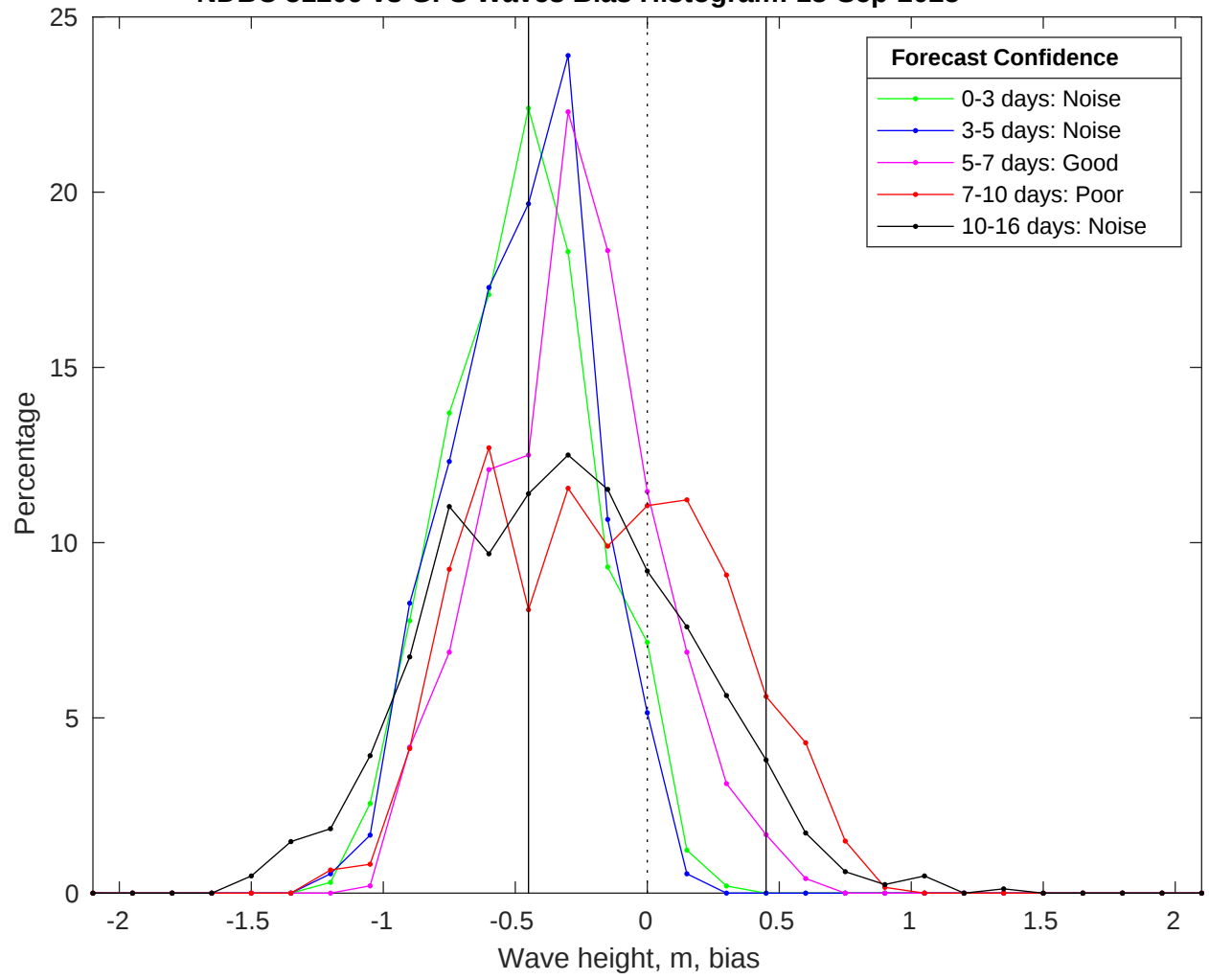
NDBC 51209 vs GFS Waves Bias Histogram: 13-Sep-2025
