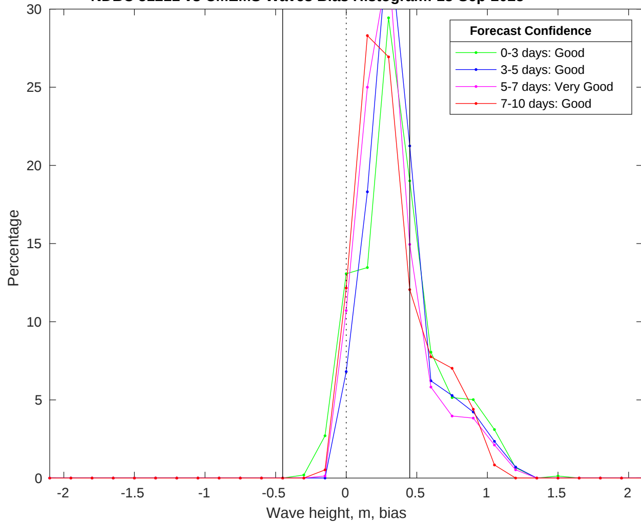
NDBC 51211 vs CMEMS Waves Bias Histogram: 13-Sep-2025
