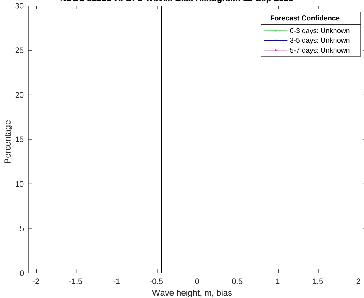
NDBC 51211 vs GFS Waves Bias Histogram: 13-Sep-2025
