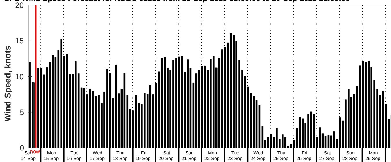
GFS Wind Speed Forecast for NDBC 52211 from 13-Sep-2025 11:00:00 to 29-Sep-2025 11:00:00
