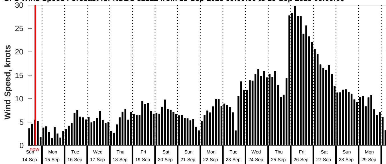
GFS Wind Speed Forecast for NDBC 52212 from 13-Sep-2025 09:00:00 to 29-Sep-2025 09:00:00
