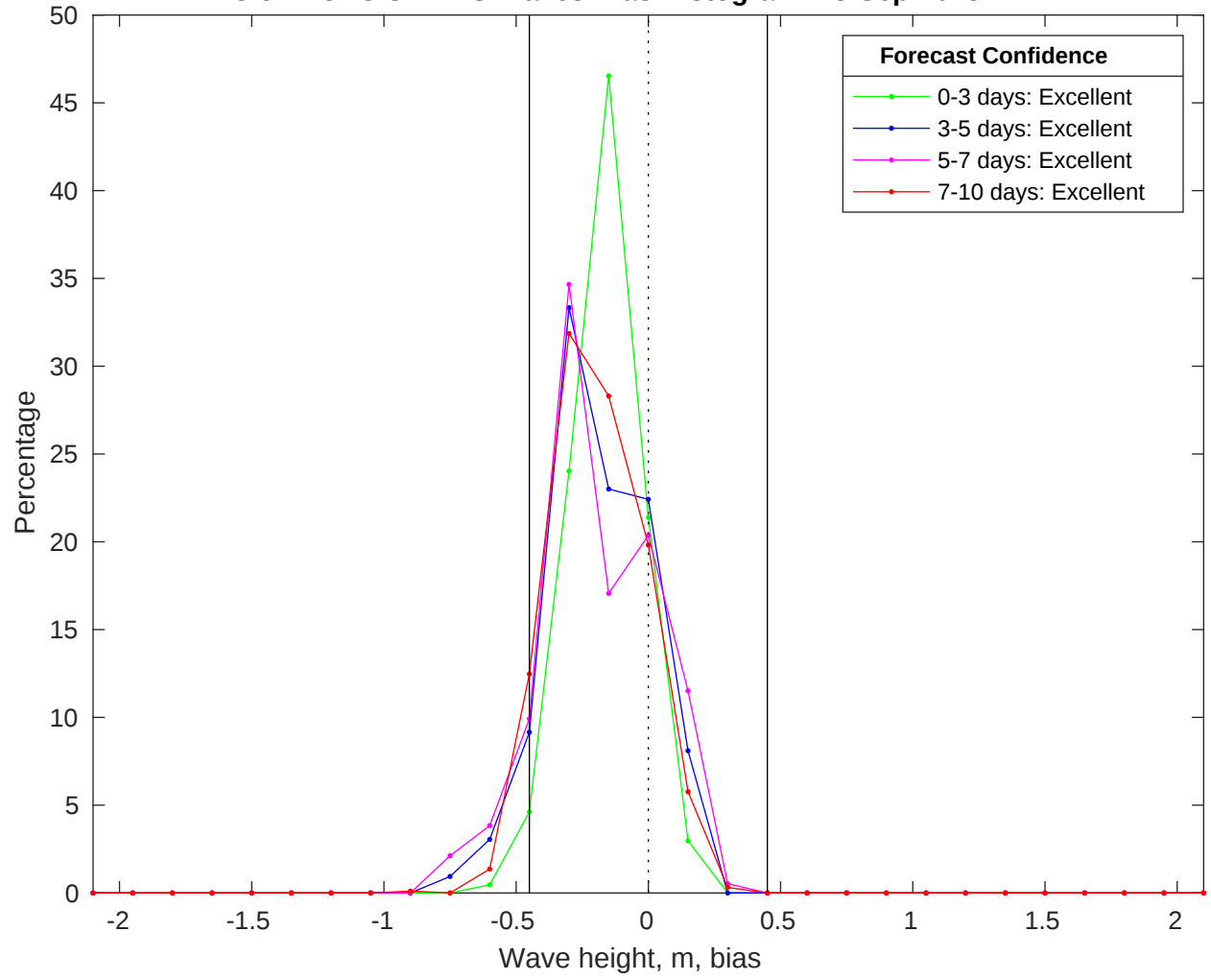
NDBC 52213 vs CMEMS Waves Bias Histogram: 13-Sep-2025
