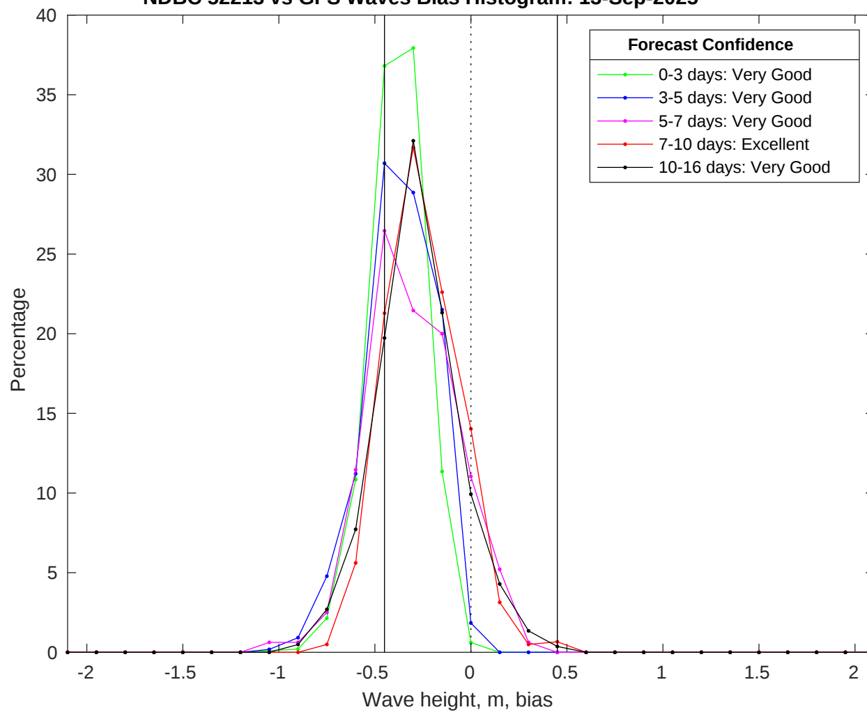
NDBC 52213 vs GFS Waves Bias Histogram: 13-Sep-2025
