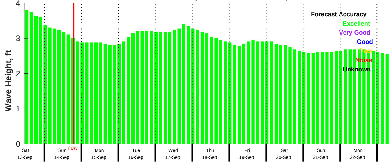
CMEMS Wave Forecast for NDBC 52213 from 12-Sep-2025 11:00:00 to 22-Sep-2025 11:00:00
