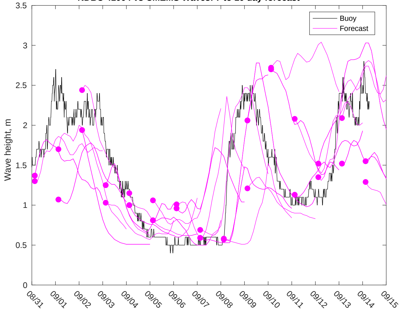
NDBC 41004 vs CMEMS Waves: 7 to 10 day forecast
