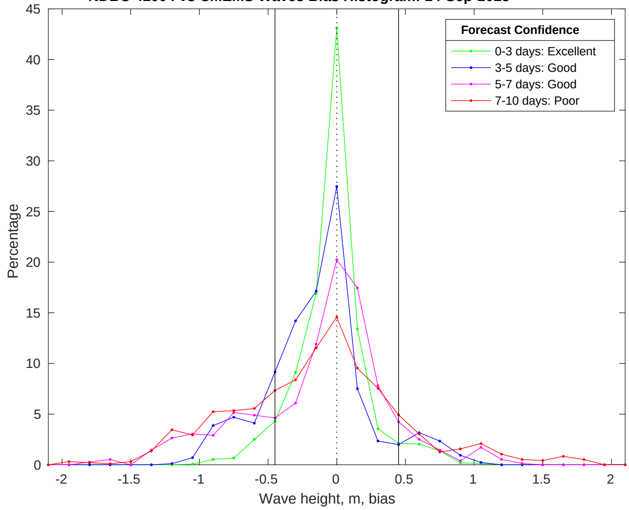
NDBC 41004 vs CMEMS Waves Bias Histogram: 14-Sep-2025
