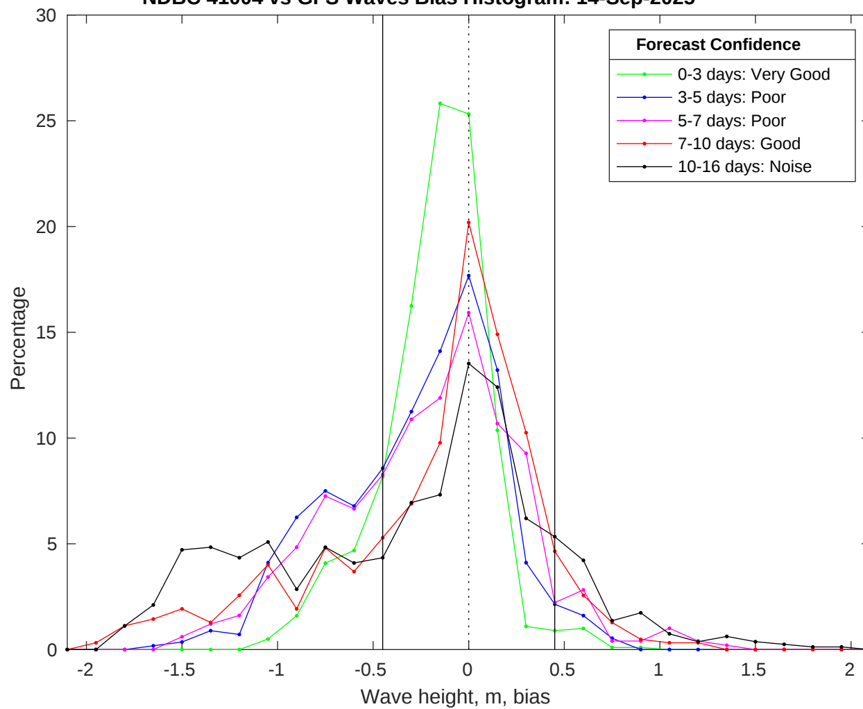
NDBC 41004 vs GFS Waves Bias Histogram: 14-Sep-2025
