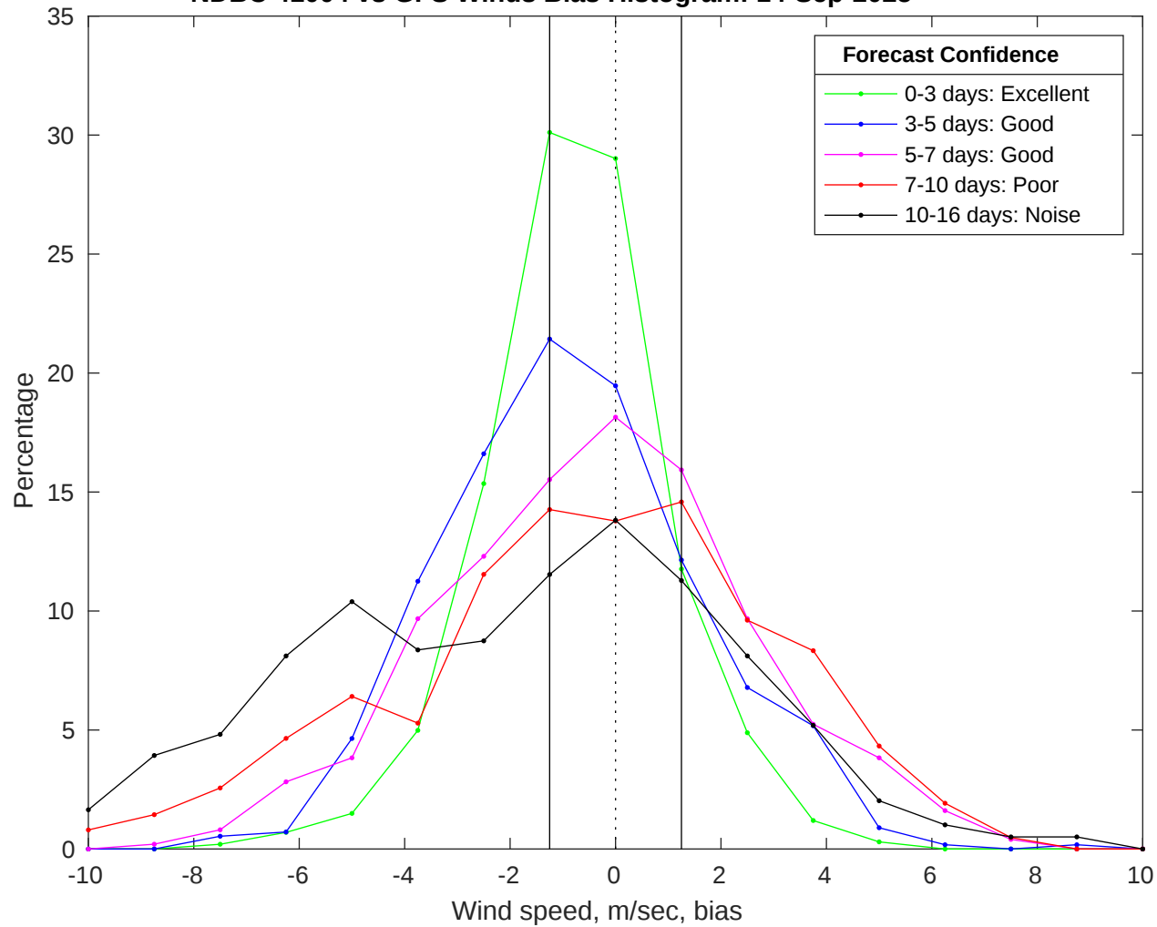
NDBC 41004 vs GFS Winds Bias Histogram: 14-Sep-2025
