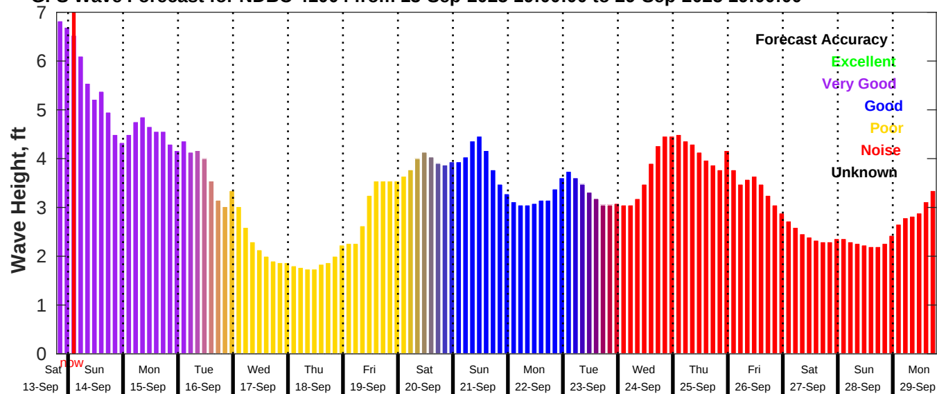
GFS Wave Forecast for NDBC 41004 from 13-Sep-2025 19:00:00 to 29-Sep-2025 19:00:00
