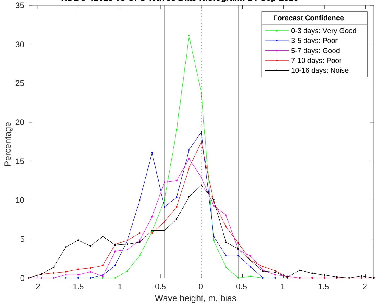
NDBC 41013 vs GFS Waves Bias Histogram: 14-Sep-2025
