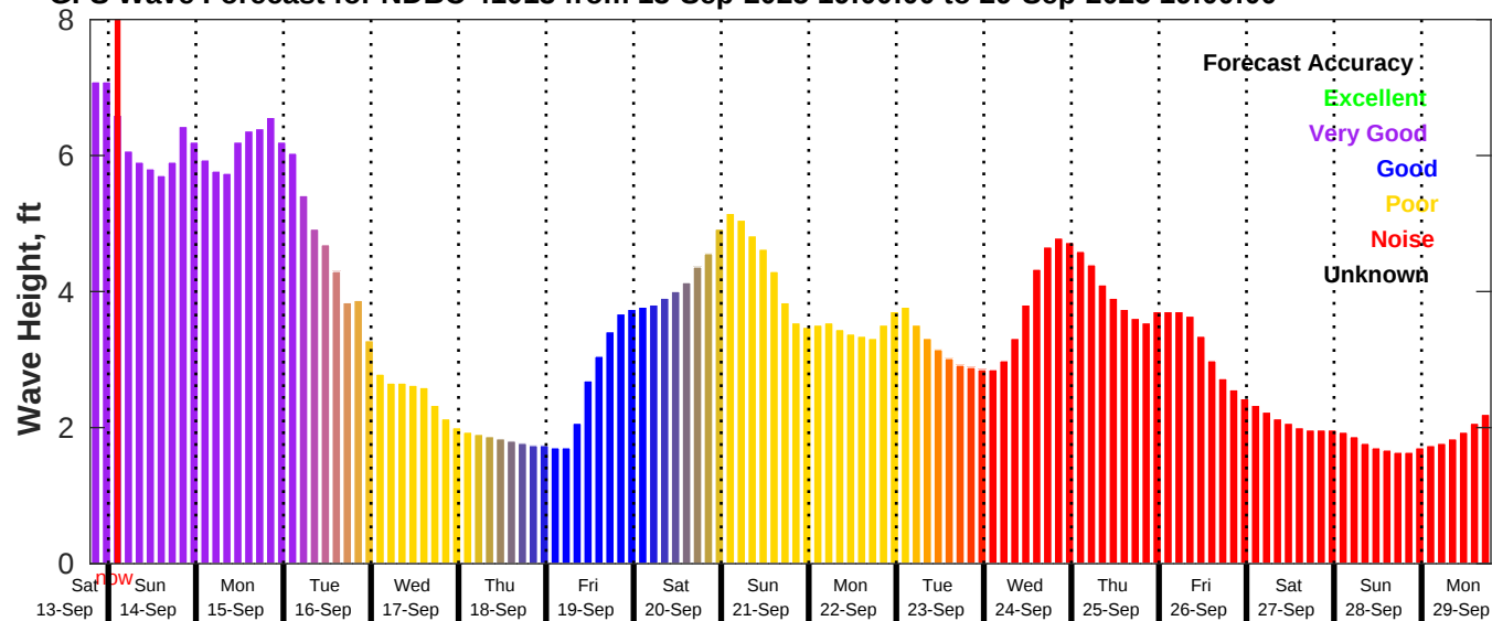
GFS Wave Forecast for NDBC 41013 from 13-Sep-2025 19:00:00 to 29-Sep-2025 19:00:00
