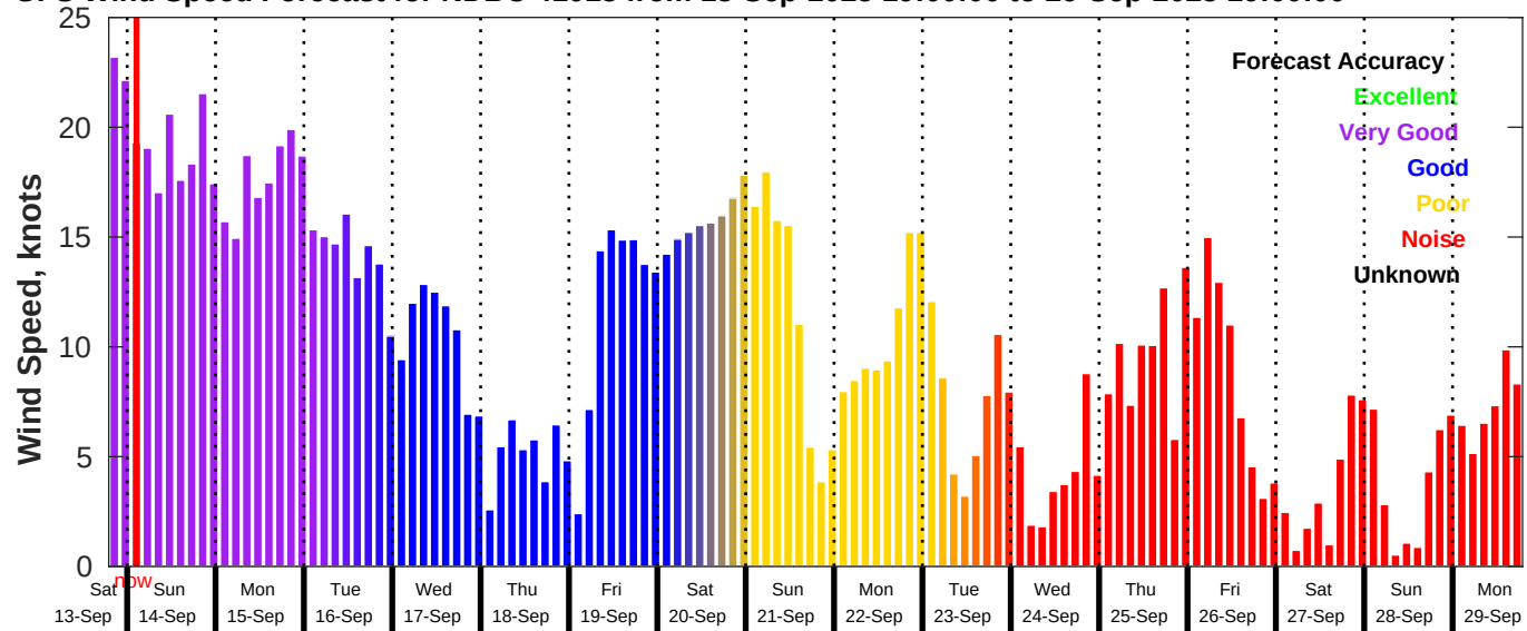
GFS Wind Speed Forecast for NDBC 41013 from 13-Sep-2025 19:00:00 to 29-Sep-2025 19:00:00
