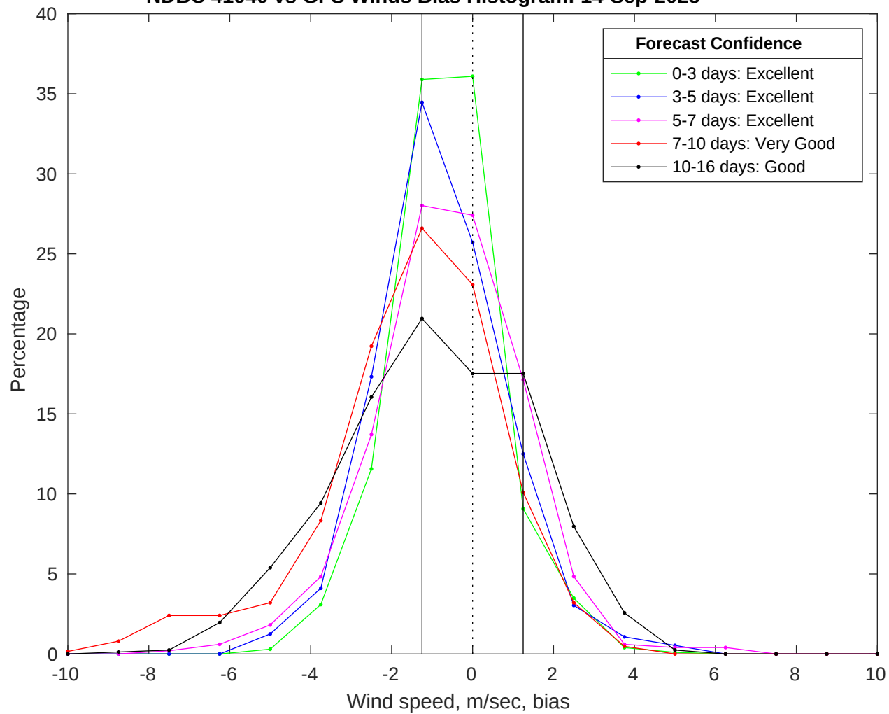
NDBC 41040 vs GFS Winds Bias Histogram: 14-Sep-2025
