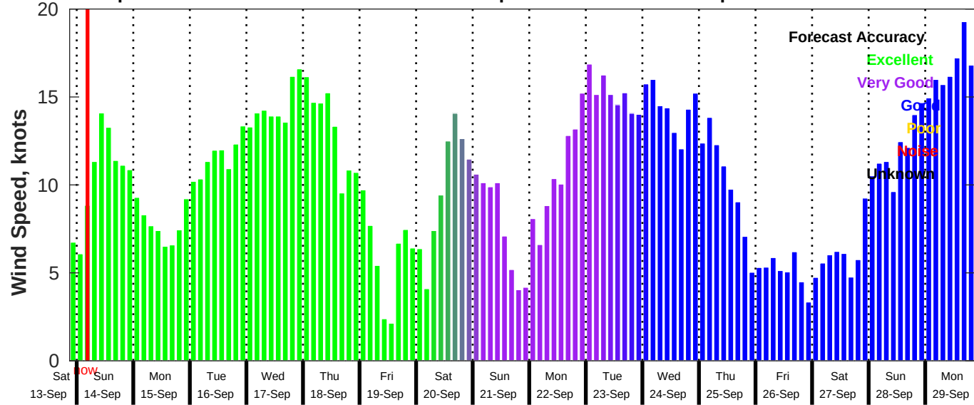
GFS Wind Speed Forecast for NDBC 41040 from 13-Sep-2025 21:00:00 to 29-Sep-2025 21:00:00
