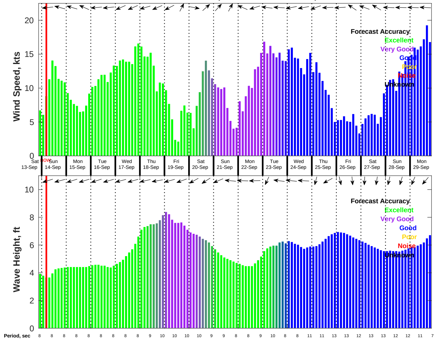
Wind & Wave Forecast for NDBC 41040 from 13-Sep-2025 21:00:00 to 29-Sep-2025 21:00:00
