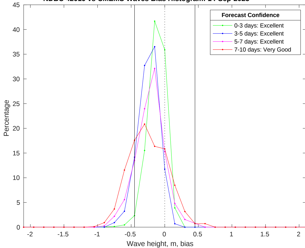
NDBC 42019 vs CMEMS Waves Bias Histogram: 14-Sep-2025
