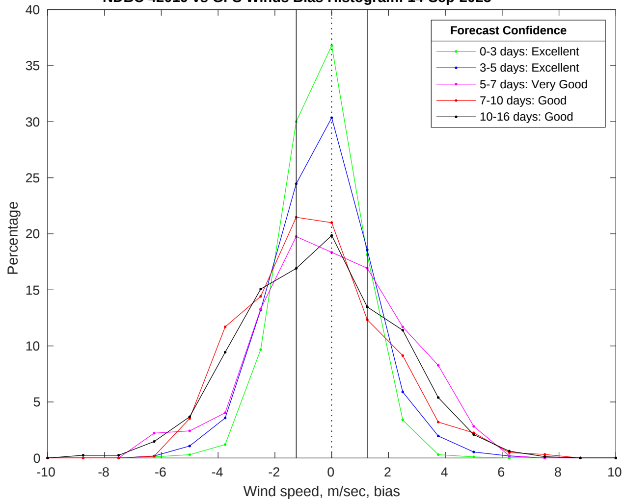
NDBC 42019 vs GFS Winds Bias Histogram: 14-Sep-2025
