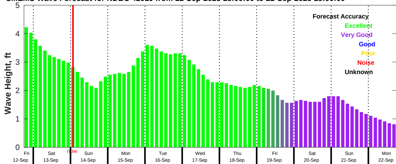
CMEMS Wave Forecast for NDBC 42019 from 12-Sep-2025 18:00:00 to 22-Sep-2025 18:00:00
