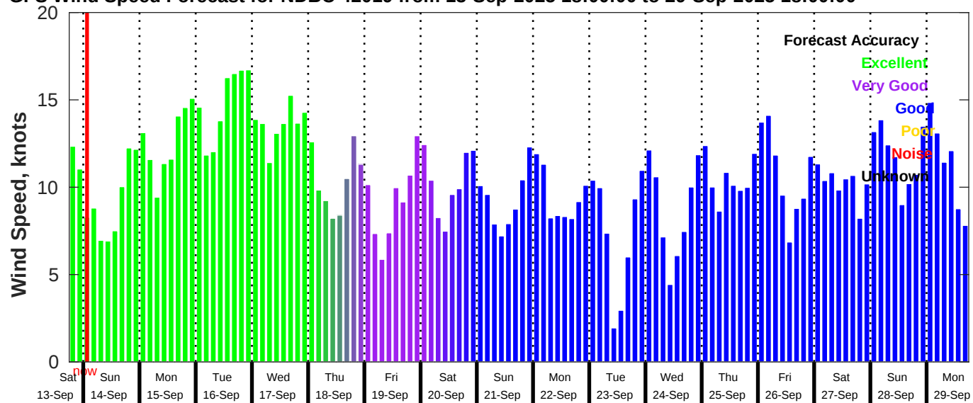
GFS Wind Speed Forecast for NDBC 42019 from 13-Sep-2025 18:00:00 to 29-Sep-2025 18:00:00
