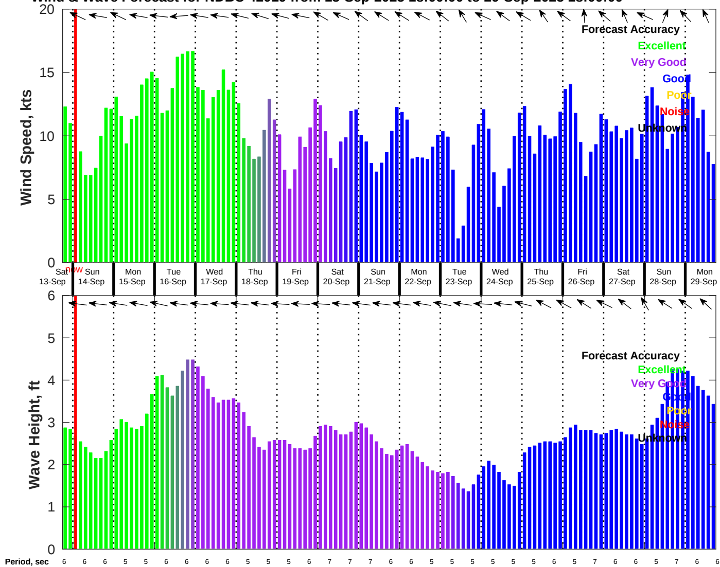
Wind & Wave Forecast for NDBC 42019 from 13-Sep-2025 18:00:00 to 29-Sep-2025 18:00:00
