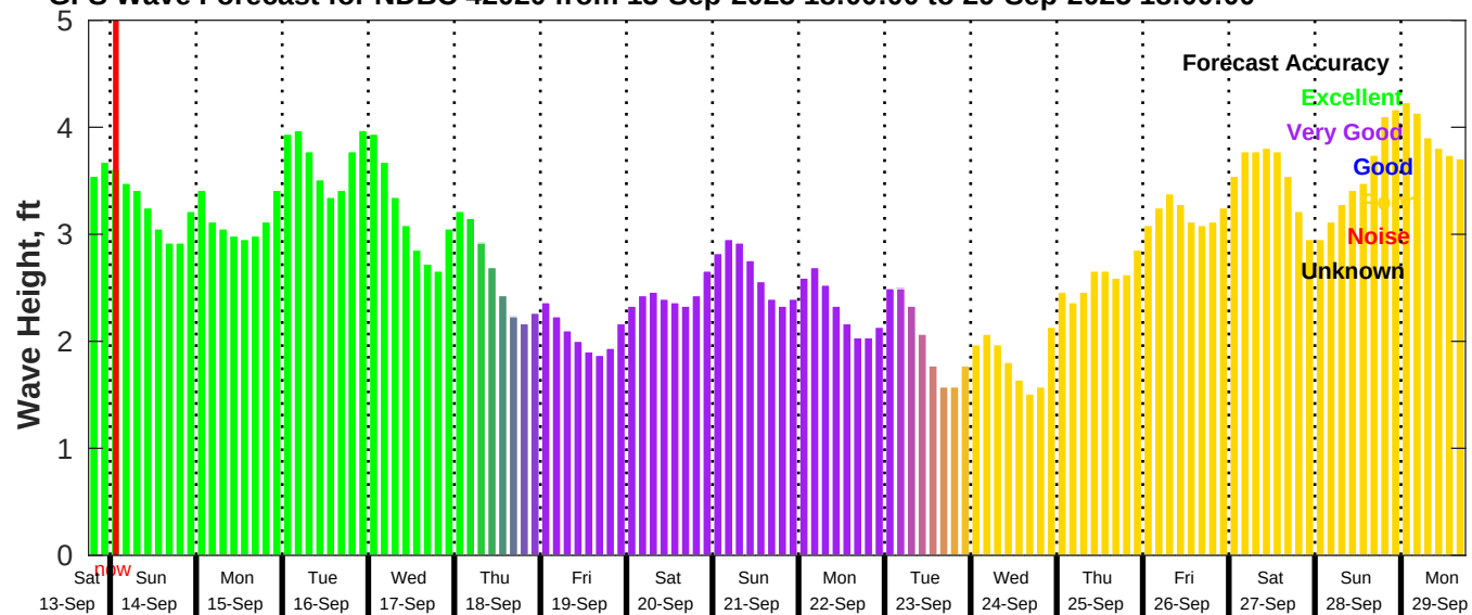
GFS Wave Forecast for NDBC 42020 from 13-Sep-2025 18:00:00 to 29-Sep-2025 18:00:00
